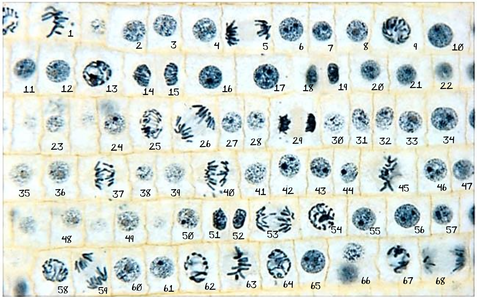
Interphase
